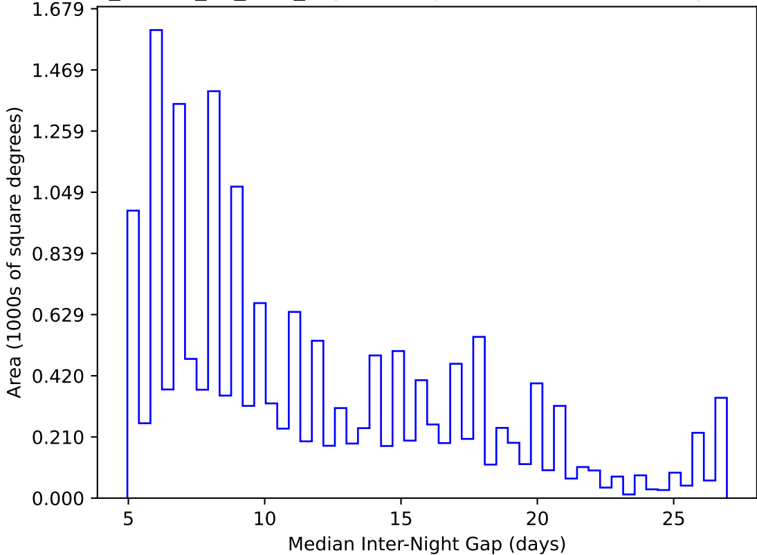
ddf_loaded_fl1_v3.4_10yrs WFD y band: Median Inter-Night Gap
