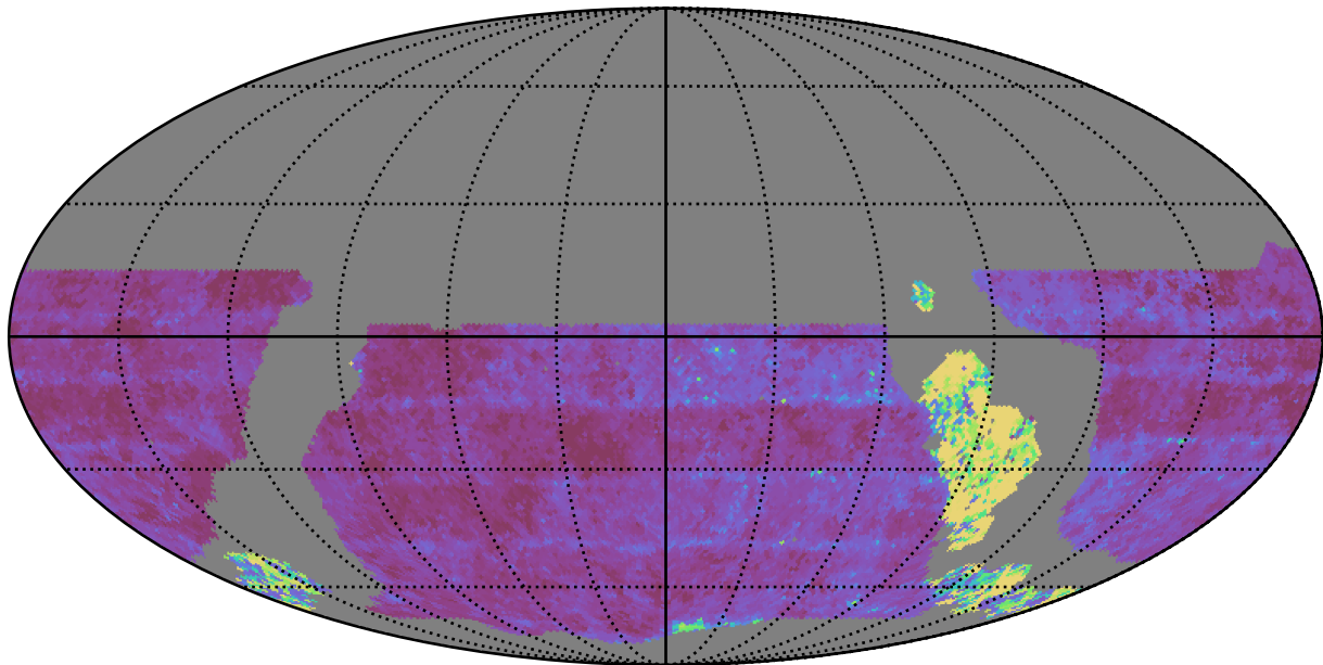
ddf_loaded_fl1_v3.4_10yrs WFD u band: Median Inter-Night Gap
