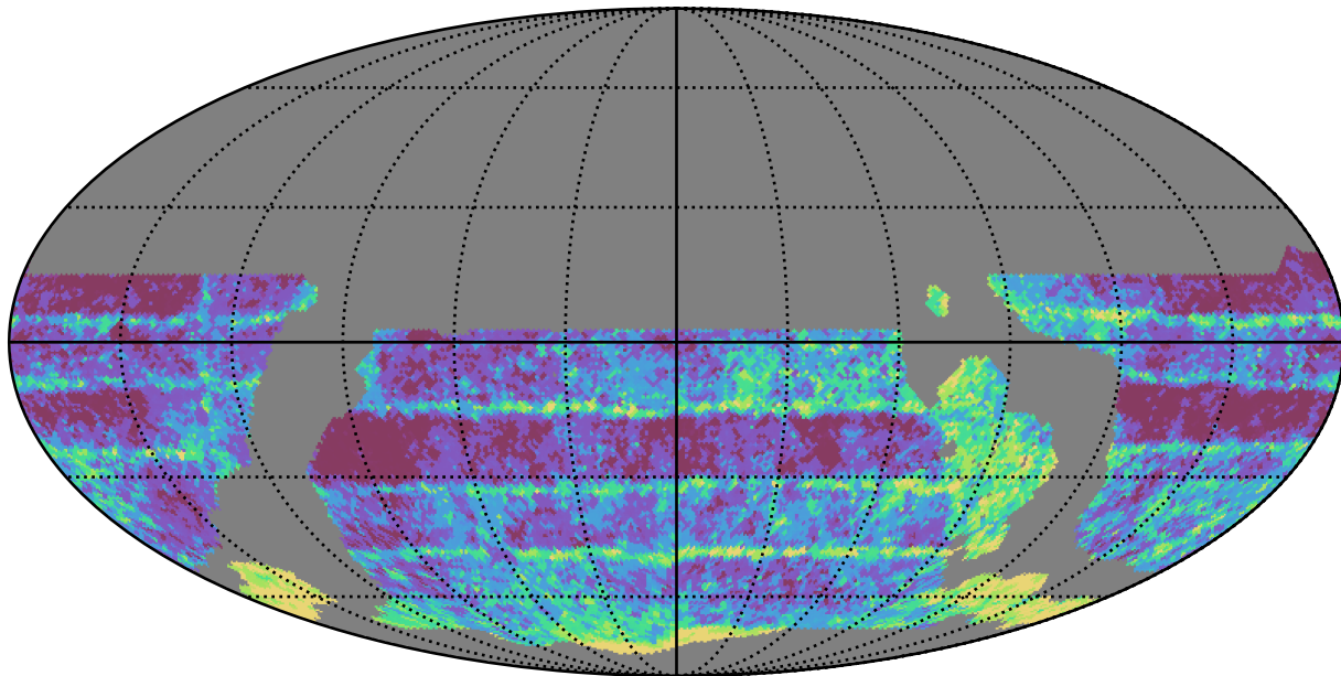
ddf_loaded_fl1_v3.4_10yrs WFD r band: Median Inter-Night Gap
