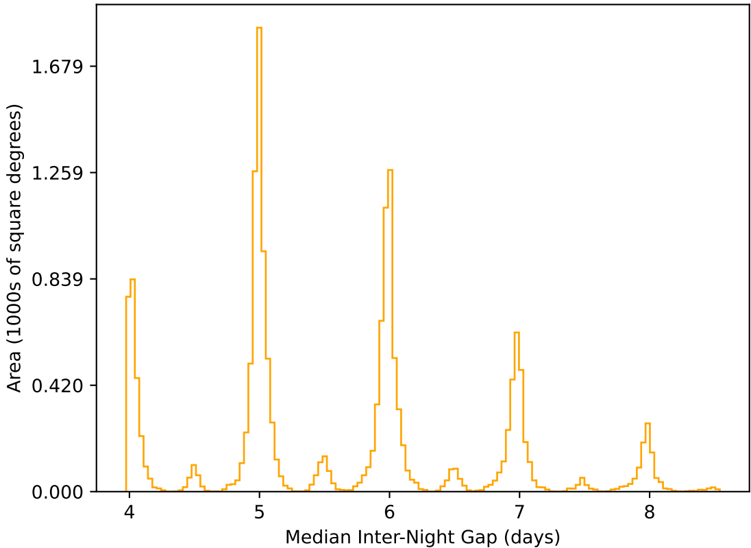
ddf_loaded_fl1_v3.4_10yrs WFD r band: Median Inter-Night Gap
