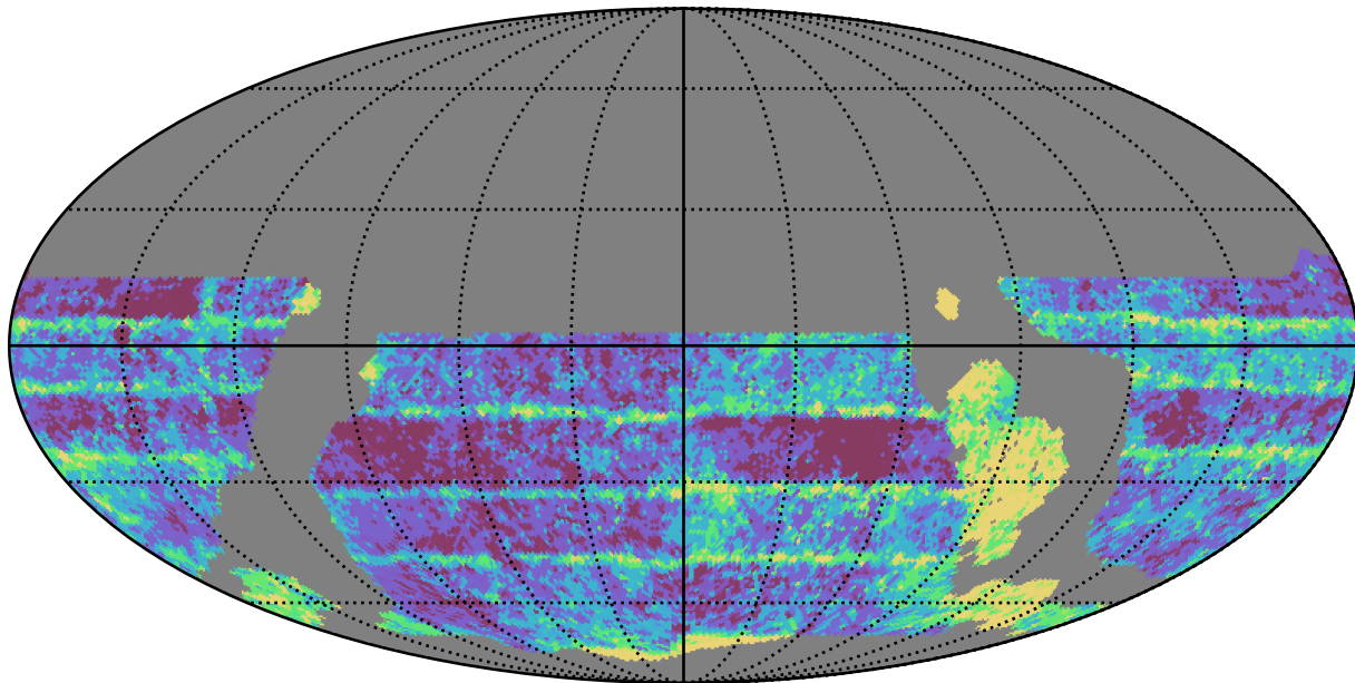
ddf_loaded_fl1_v3.4_10yrs WFD i band: Median Inter-Night Gap
