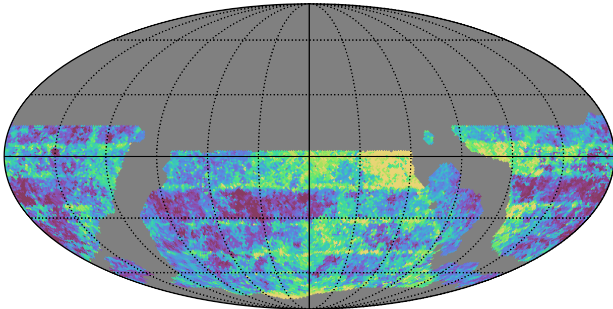
ddf_loaded_fl1_v3.4_10yrs WFD g band: Median Inter-Night Gap
