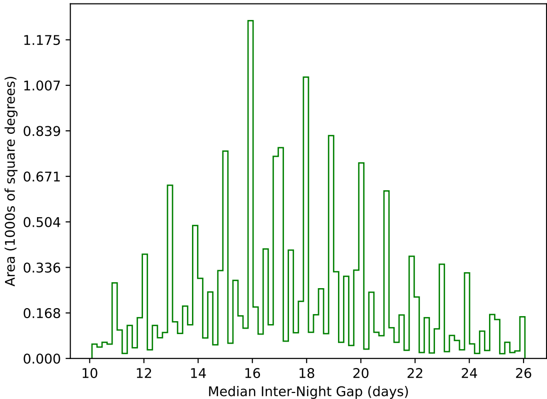
ddf_loaded_fl1_v3.4_10yrs WFD g band: Median Inter-Night Gap
