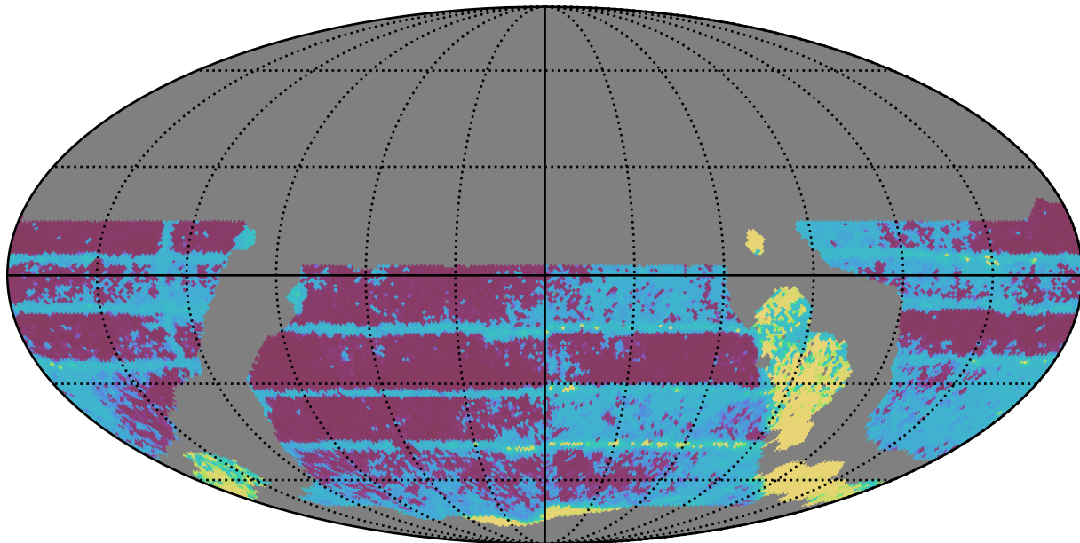
ddf_loaded_fl1_v3.4_10yrs WFD all bands: Median Inter-Night Gap
