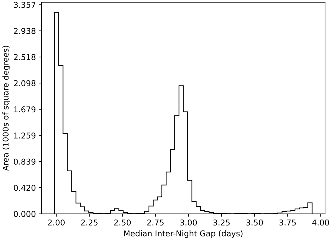
ddf_loaded_fl1_v3.4_10yrs WFD all bands: Median Inter-Night Gap
