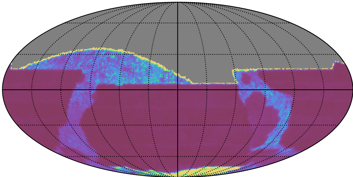
ddf_loaded_fl1_v3.4_10yrs All sky z band: Median Inter-Night Gap
