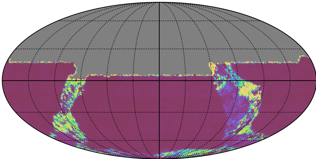
ddf_loaded_fl1_v3.4_10yrs All sky u band: Median Inter-Night Gap
