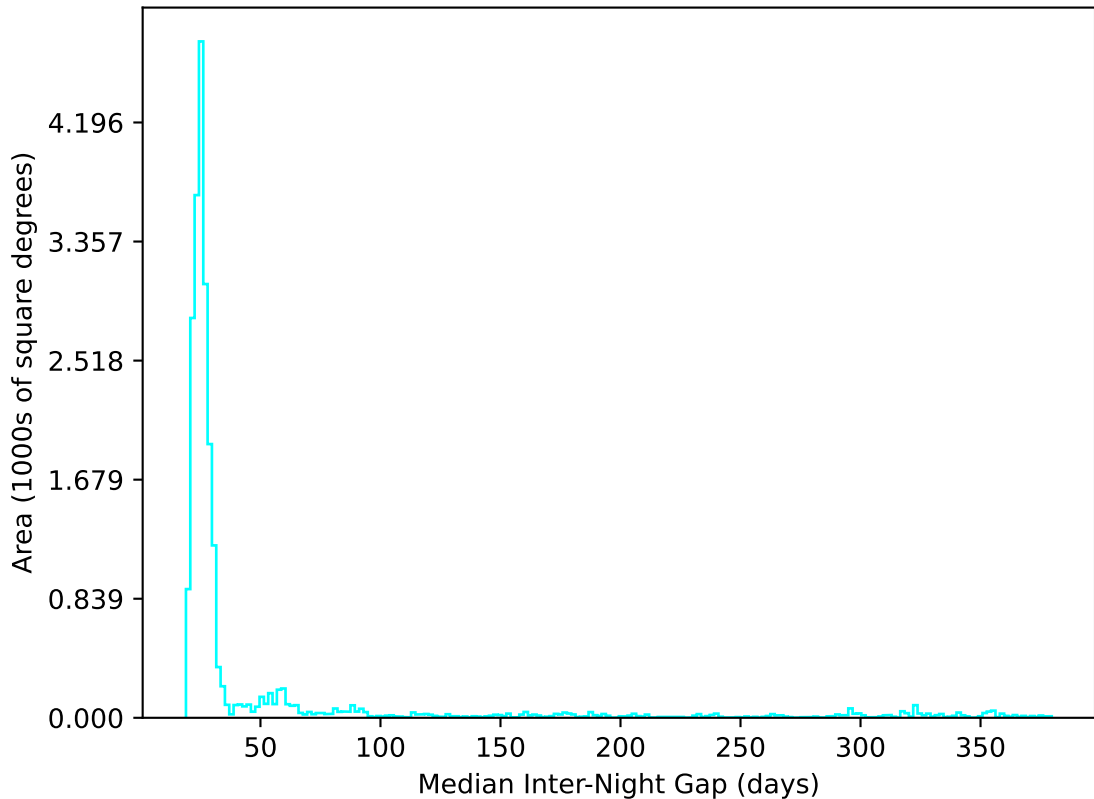
ddf_loaded_fl1_v3.4_10yrs All sky u band: Median Inter-Night Gap
