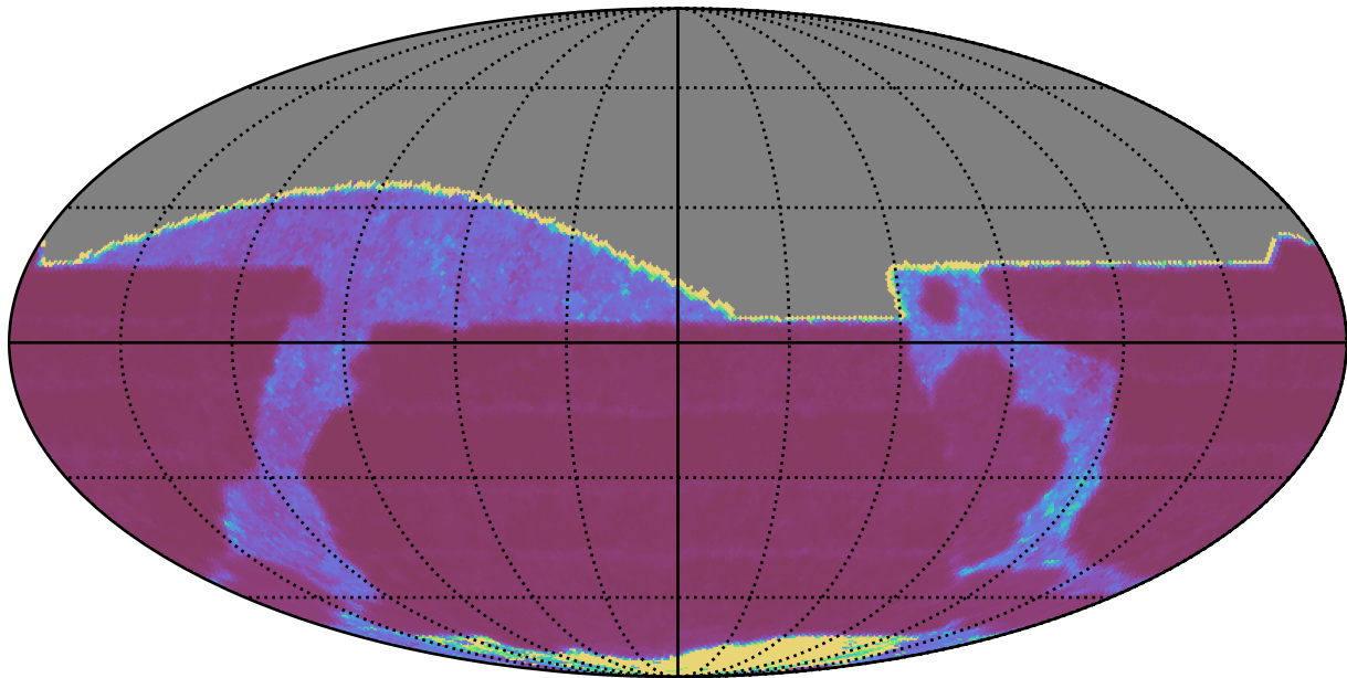
ddf_loaded_fl1_v3.4_10yrs All sky r band: Median Inter-Night Gap
