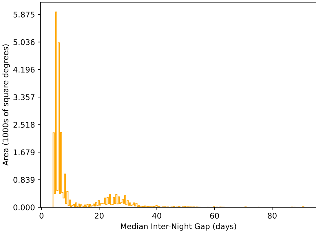
ddf_loaded_fl1_v3.4_10yrs All sky r band: Median Inter-Night Gap
