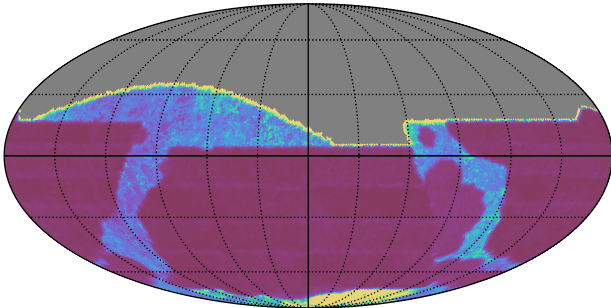
ddf_loaded_fl1_v3.4_10yrs All sky i band: Median Inter-Night Gap
