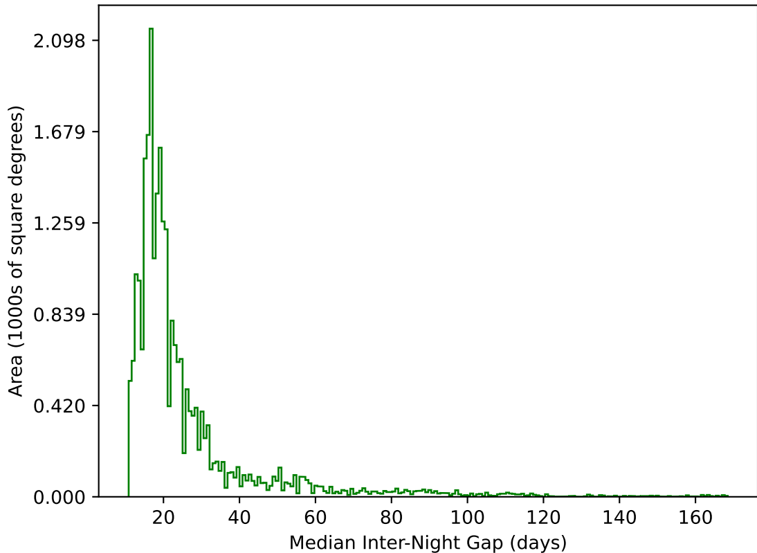
ddf_loaded_fl1_v3.4_10yrs All sky g band: Median Inter-Night Gap
