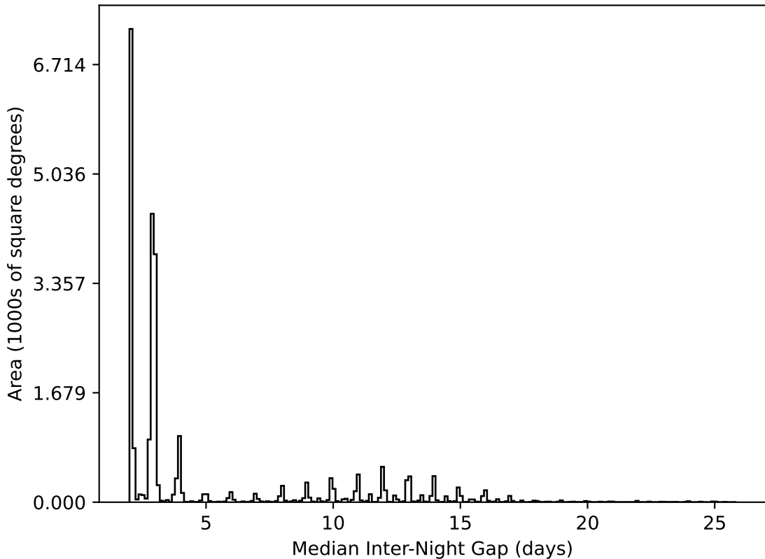
ddf_loaded_fl1_v3.4_10yrs All sky all bands: Median Inter-Night Gap
