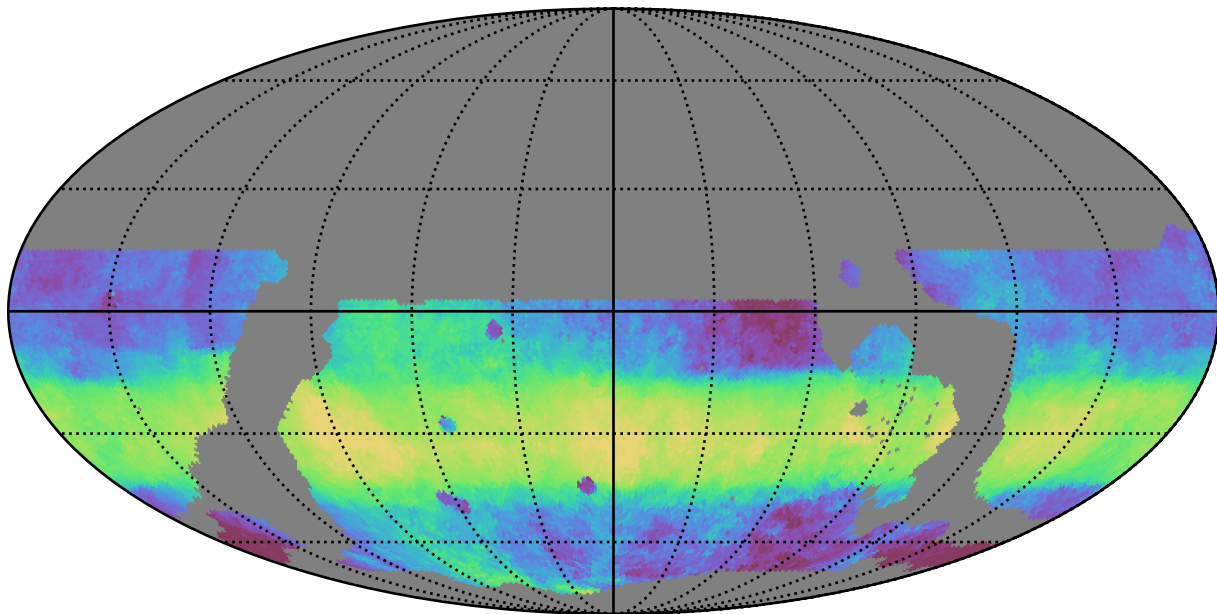
ddf_loaded_fl1_v3.4_10yrs WFD z band: Median HA
