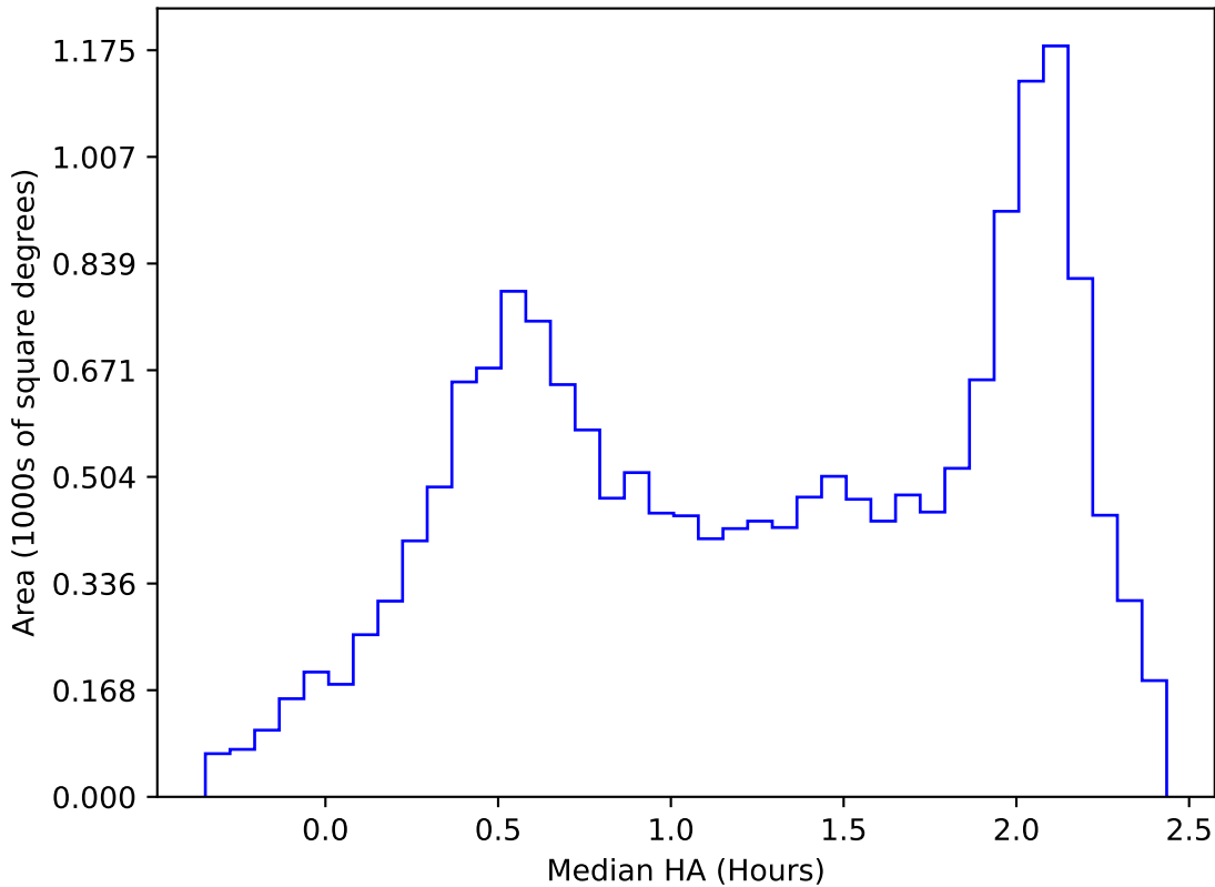
ddf_loaded_fl1_v3.4_10yrs WFD y band: Median HA
