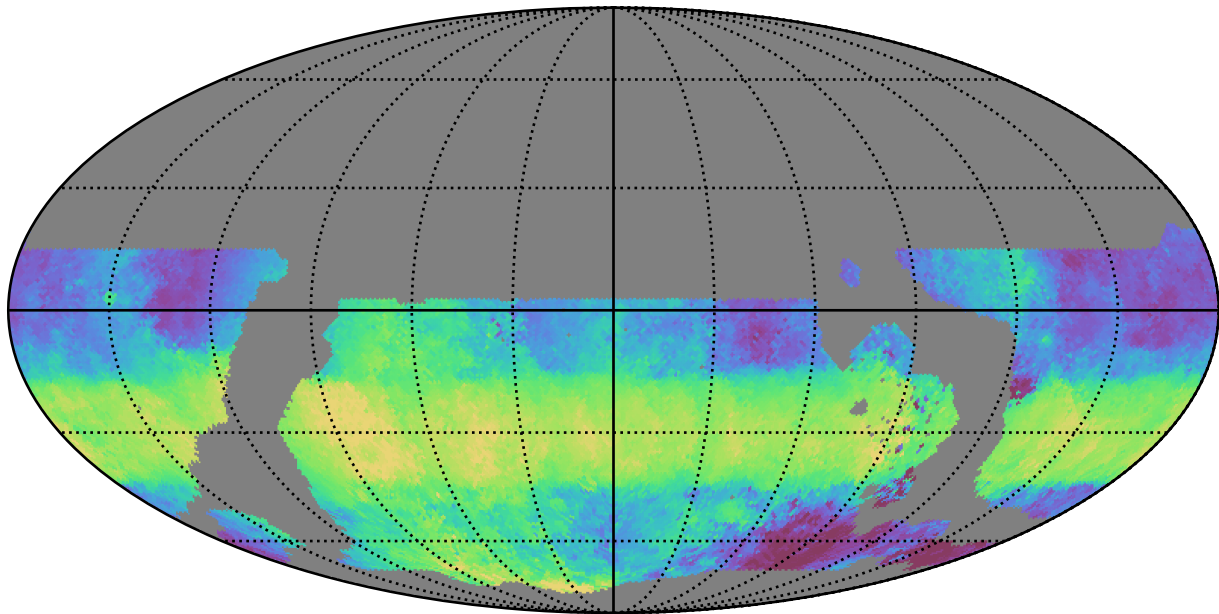
ddf_loaded_fl1_v3.4_10yrs WFD u band: Median HA
