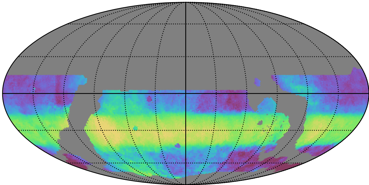
ddf_loaded_fl1_v3.4_10yrs WFD r band: Median HA
