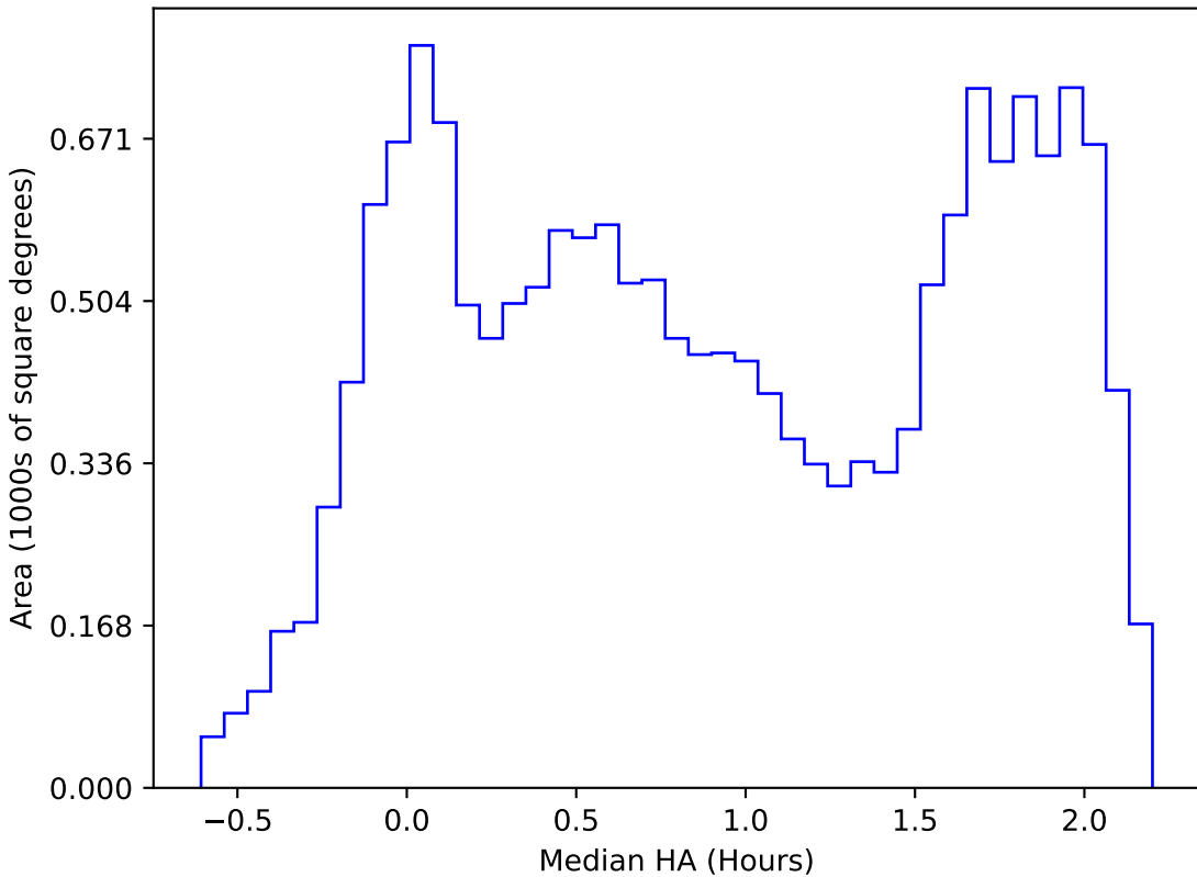
ddf_loaded_fl1_v3.4_10yrs WFD r band: Median HA
