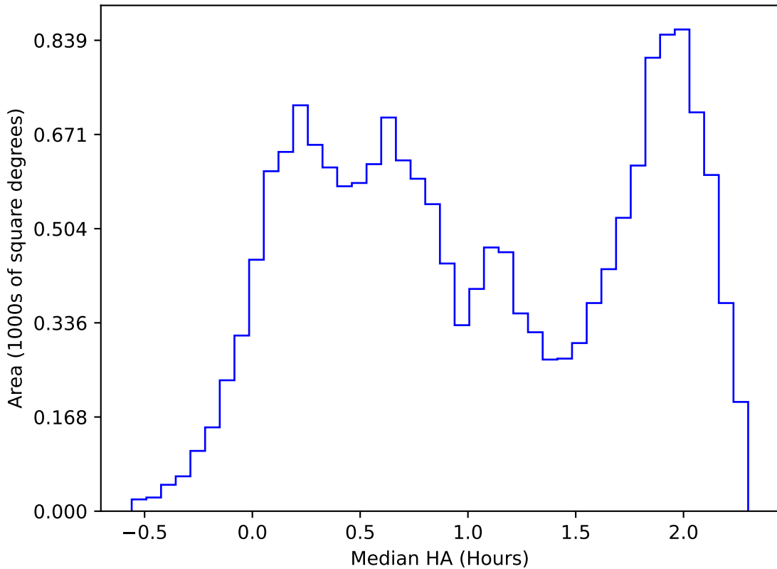
ddf_loaded_fl1_v3.4_10yrs WFD i band: Median HA
