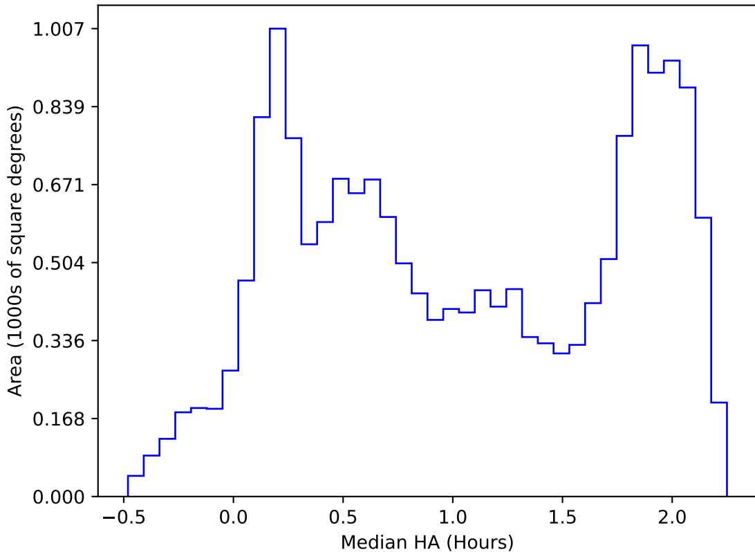
ddf_loaded_fl1_v3.4_10yrs WFD all bands: Median HA
