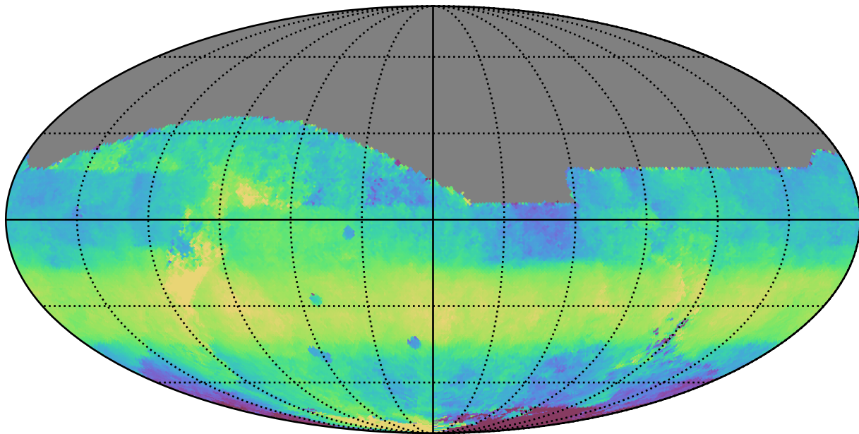
ddf_loaded_fl1_v3.4_10yrs All sky z band: Median HA
