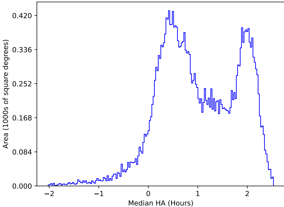
ddf_loaded_fl1_v3.4_10yrs All sky z band: Median HA
