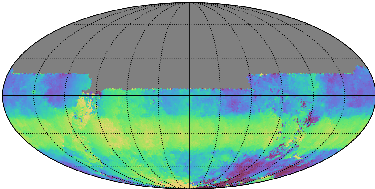
ddf_loaded_fl1_v3.4_10yrs All sky u band: Median HA
