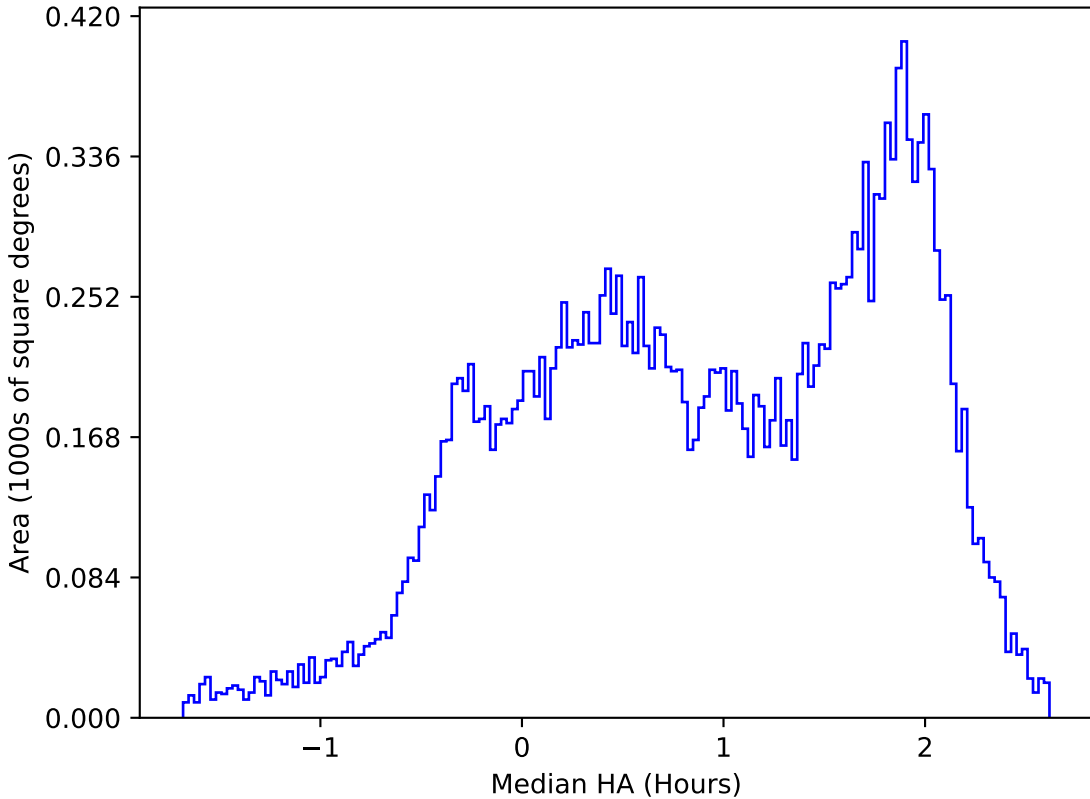
ddf_loaded_fl1_v3.4_10yrs All sky u band: Median HA
