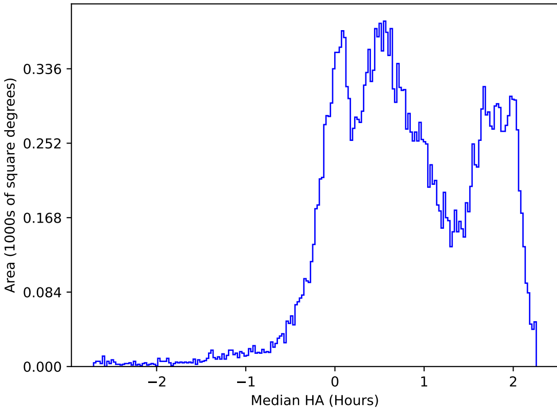
ddf_loaded_fl1_v3.4_10yrs All sky r band: Median HA
