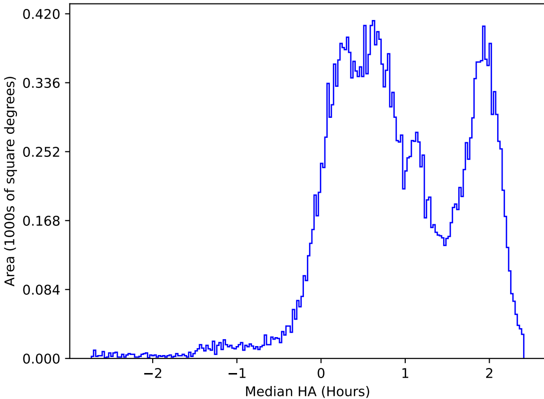
ddf_loaded_fl1_v3.4_10yrs All sky i band: Median HA
