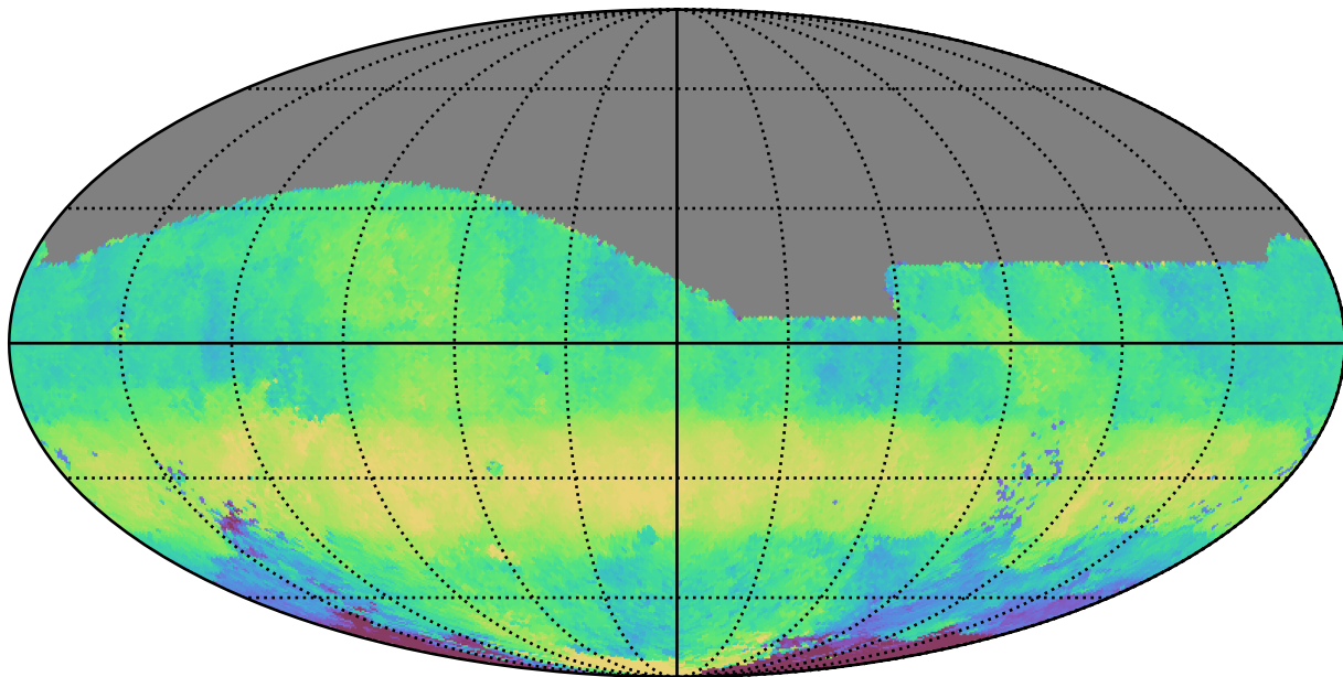
ddf_loaded_fl1_v3.4_10yrs All sky g band: Median HA
