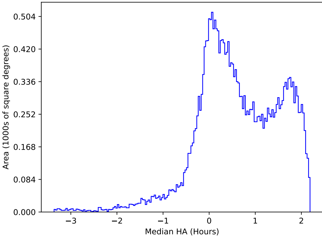
ddf_loaded_fl1_v3.4_10yrs All sky g band: Median HA
