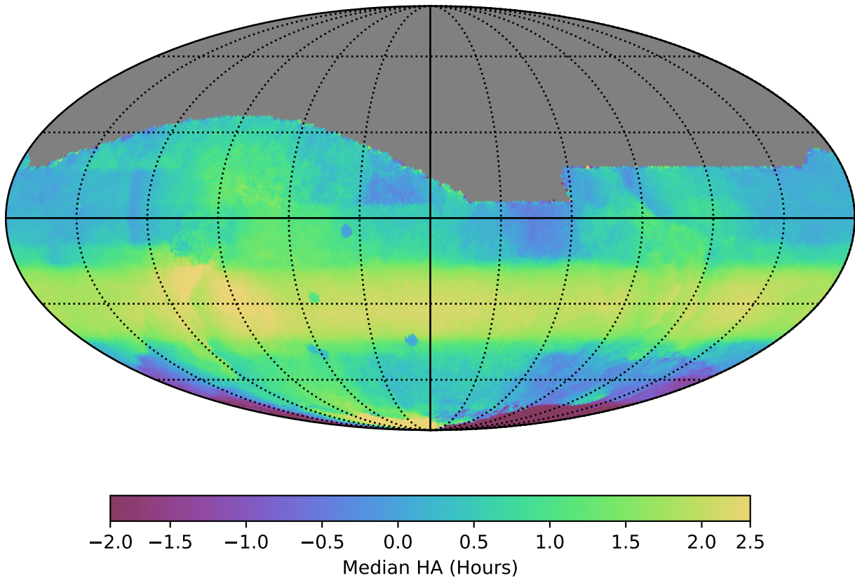
ddf_loaded_fl1_v3.4_10yrs All sky all bands: Median HA
