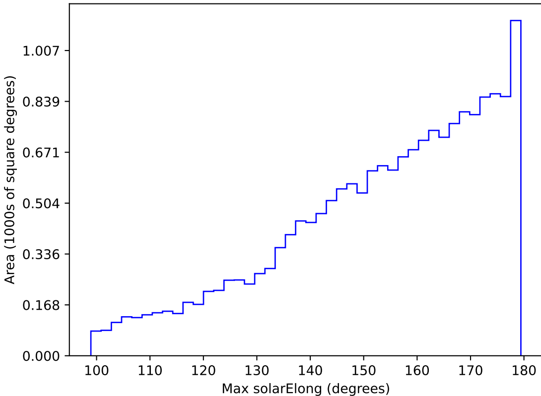
ddf_loaded_fl1_v3.4_10yrs WFD z band: Max solarElong
