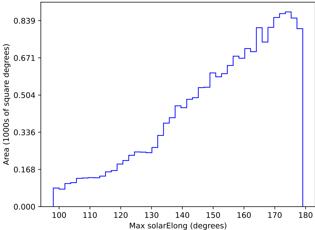
ddf_loaded_fl1_v3.4_10yrs WFD u band: Max solarElong
