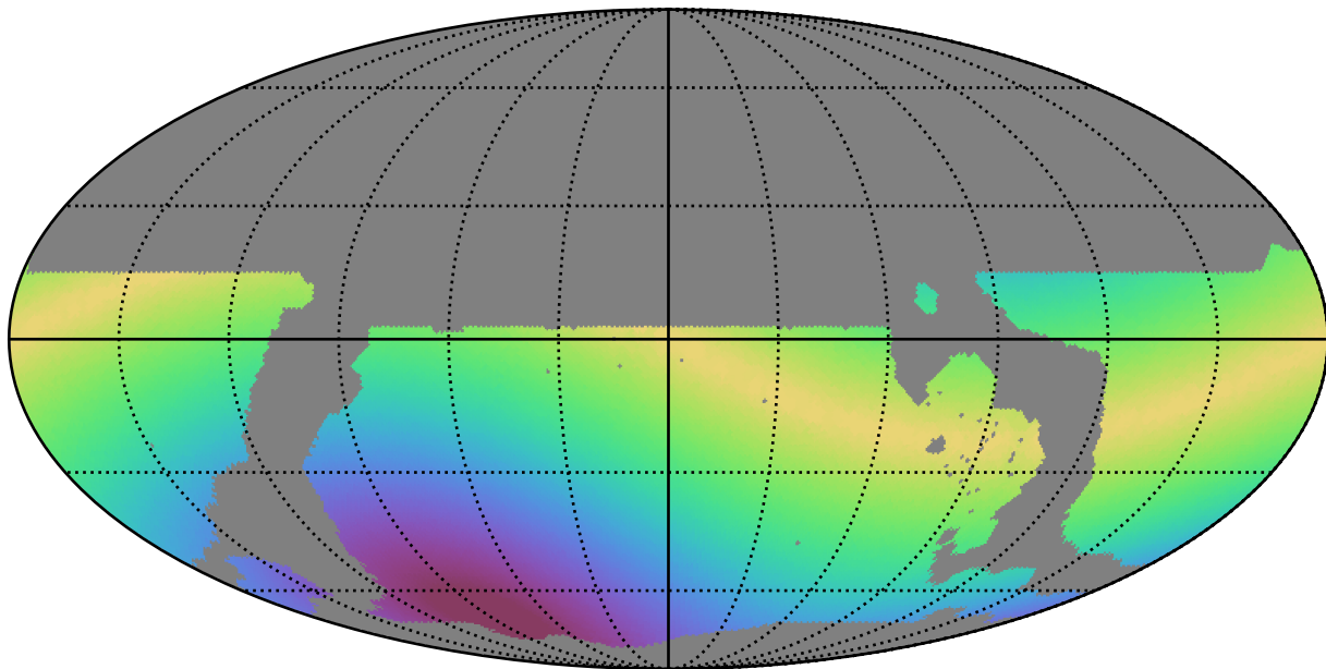
ddf_loaded_fl1_v3.4_10yrs WFD r band: Max solarElong
