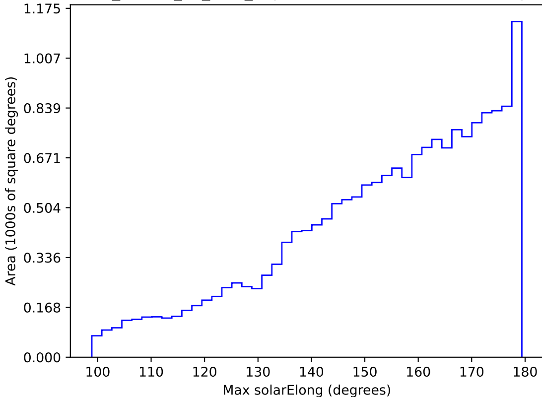
ddf_loaded_fl1_v3.4_10yrs WFD r band: Max solarElong
