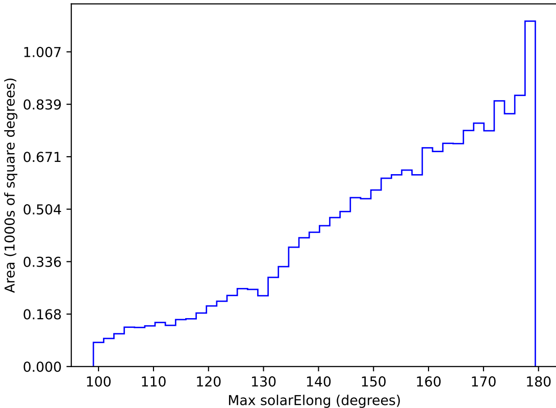
ddf_loaded_fl1_v3.4_10yrs WFD i band: Max solarElong
