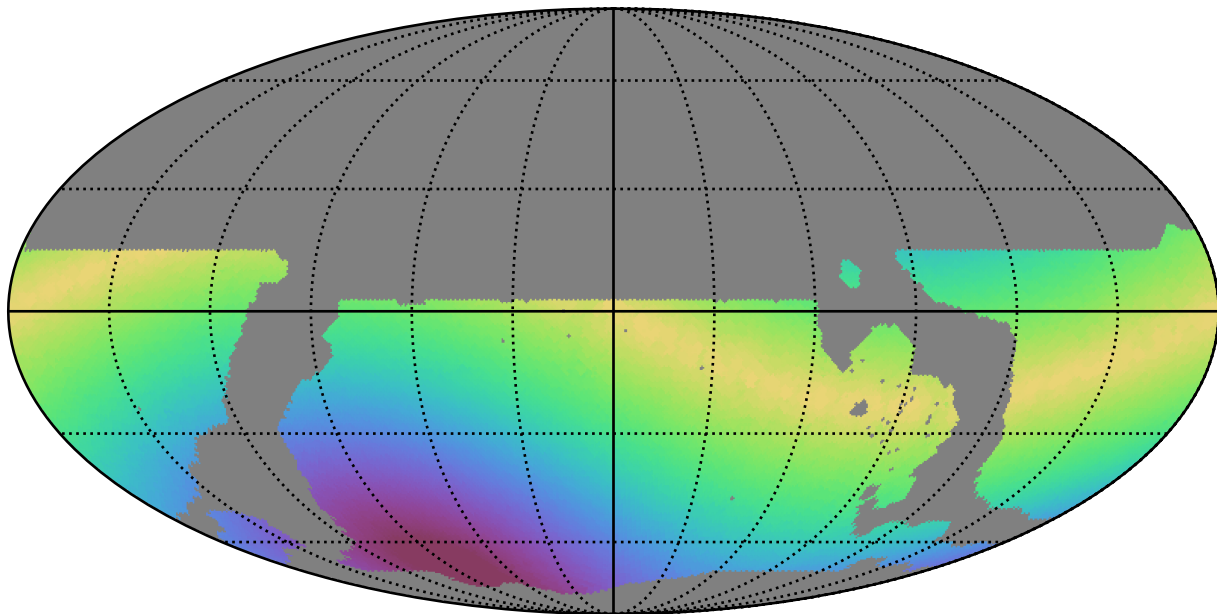
ddf_loaded_fl1_v3.4_10yrs WFD g band: Max solarElong
