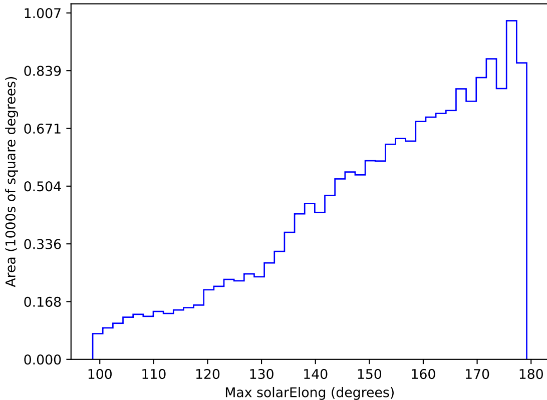
ddf_loaded_fl1_v3.4_10yrs WFD g band: Max solarElong
