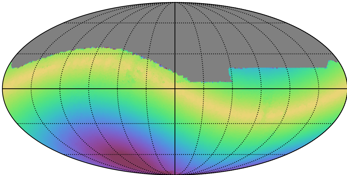
ddf_loaded_fl1_v3.4_10yrs All sky z band: Max solarElong
