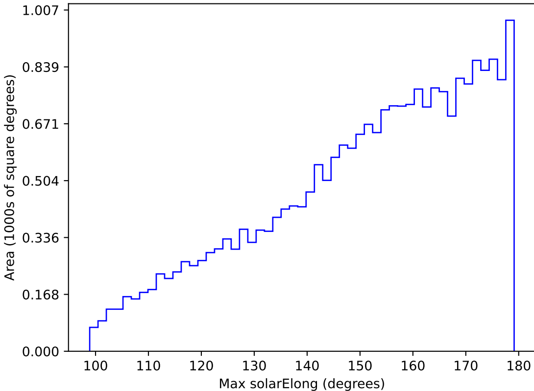
ddf_loaded_fl1_v3.4_10yrs All sky y band: Max solarElong
