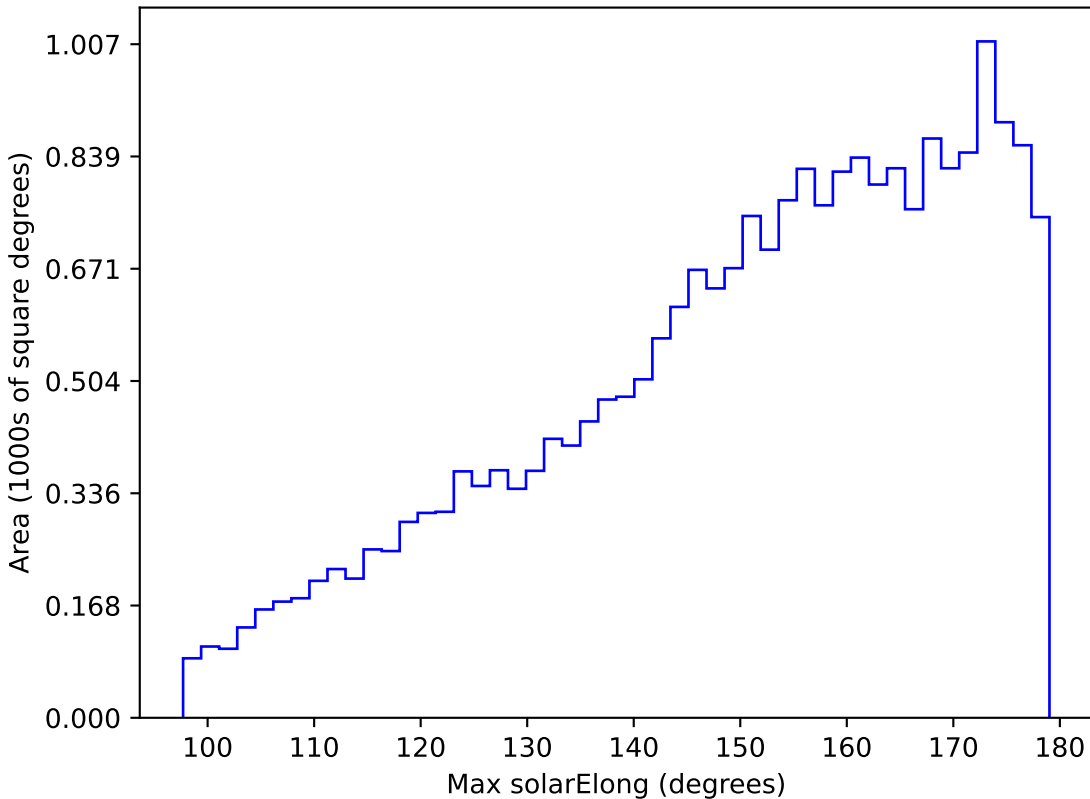
ddf_loaded_fl1_v3.4_10yrs All sky u band: Max solarElong
