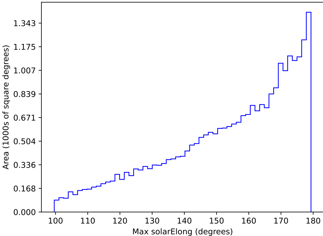
ddf_loaded_fl1_v3.4_10yrs All sky r band: Max solarElong
