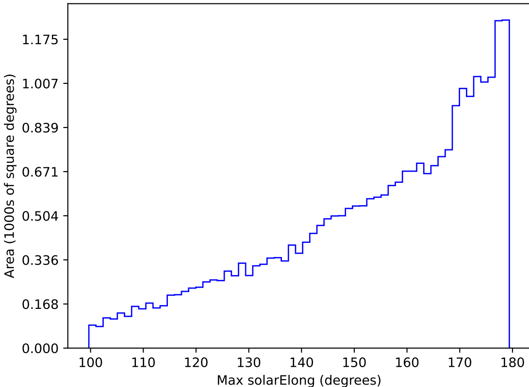
ddf_loaded_fl1_v3.4_10yrs All sky i band: Max solarElong
