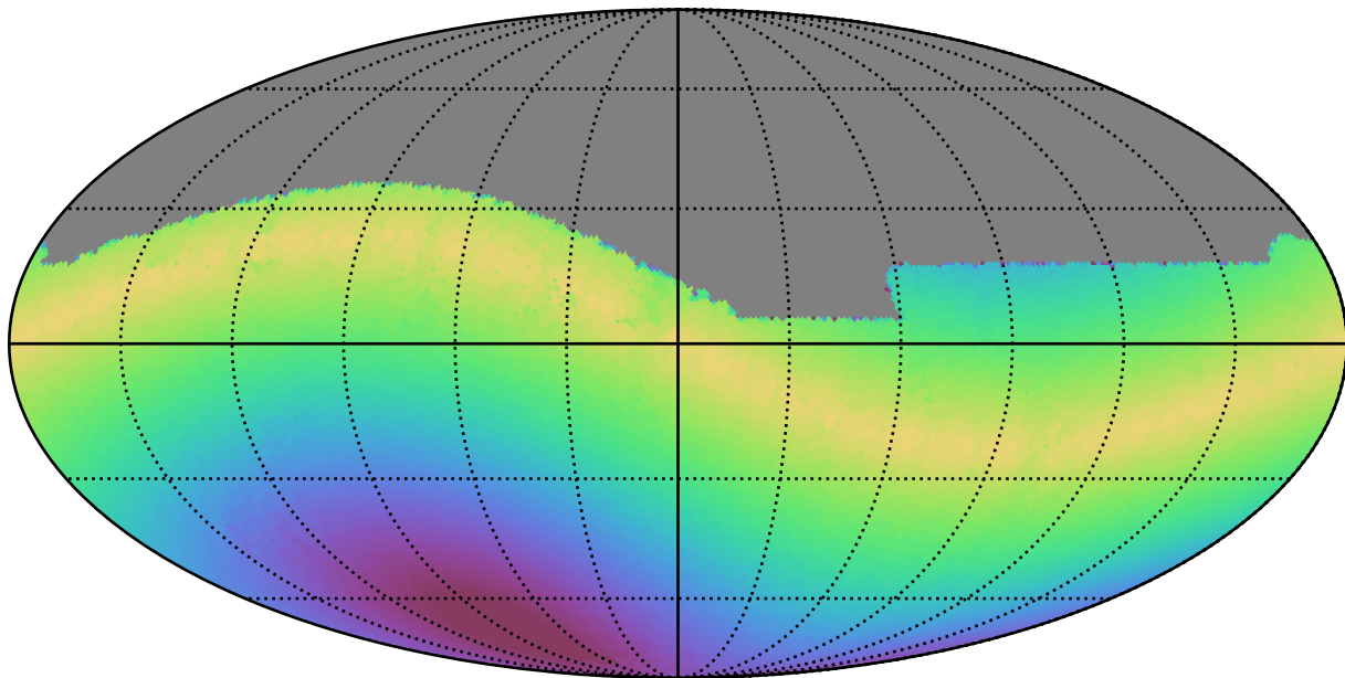
ddf_loaded_fl1_v3.4_10yrs All sky g band: Max solarElong
