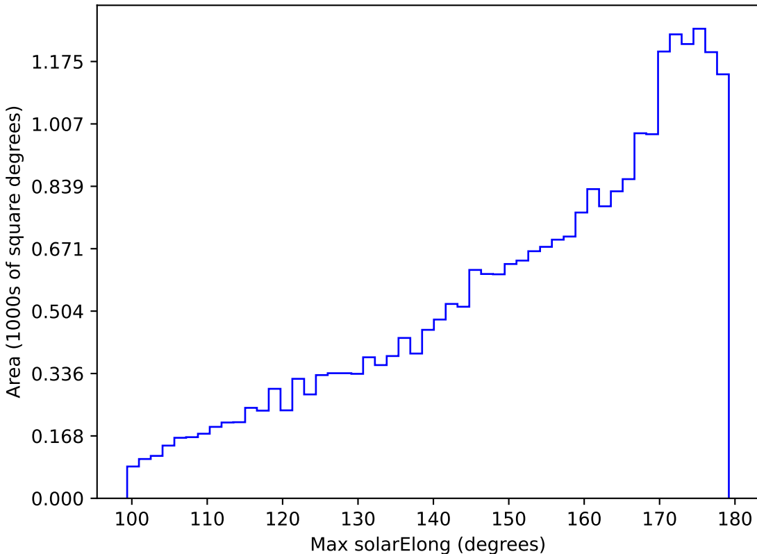
ddf_loaded_fl1_v3.4_10yrs All sky g band: Max solarElong
