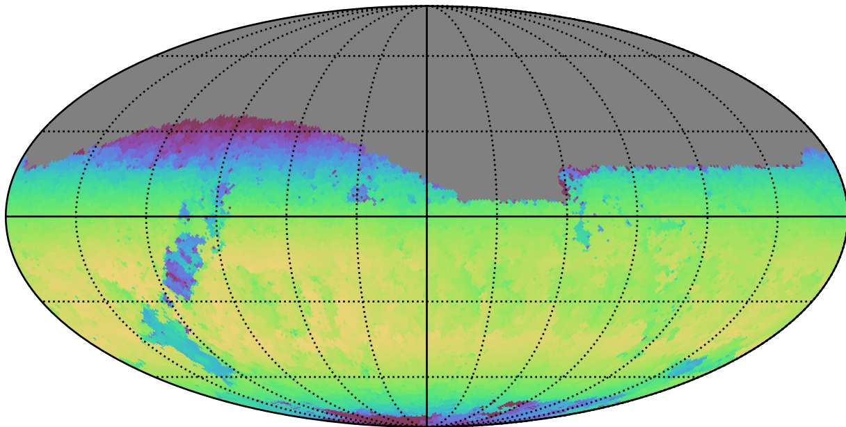
ddf_loaded_fl1_v3.4_10yrs Yr 1 z band: Max skyBrightness
