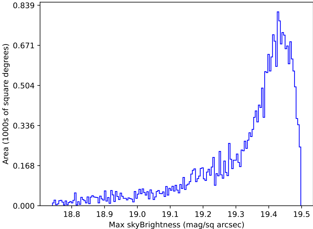
ddf_loaded_fl1_v3.4_10yrs Yr 1 z band: Max skyBrightness
