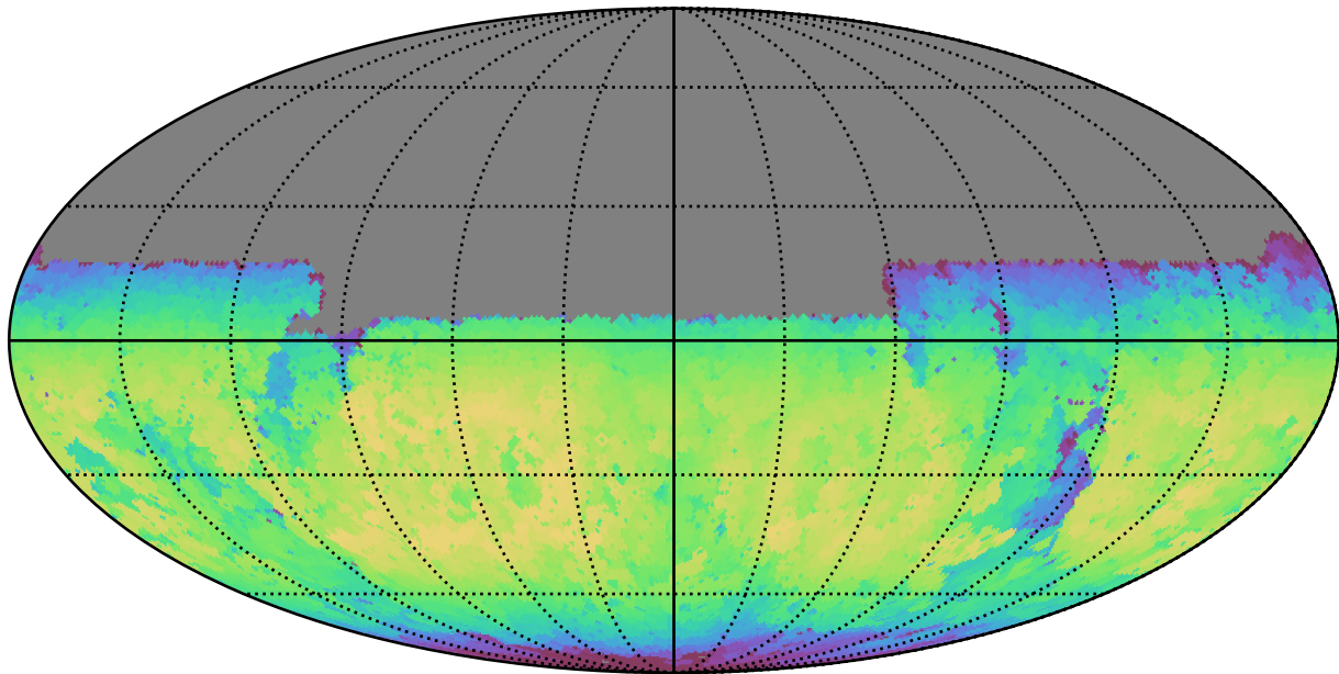
ddf_loaded_fl1_v3.4_10yrs Yr 1 y band: Max skyBrightness
